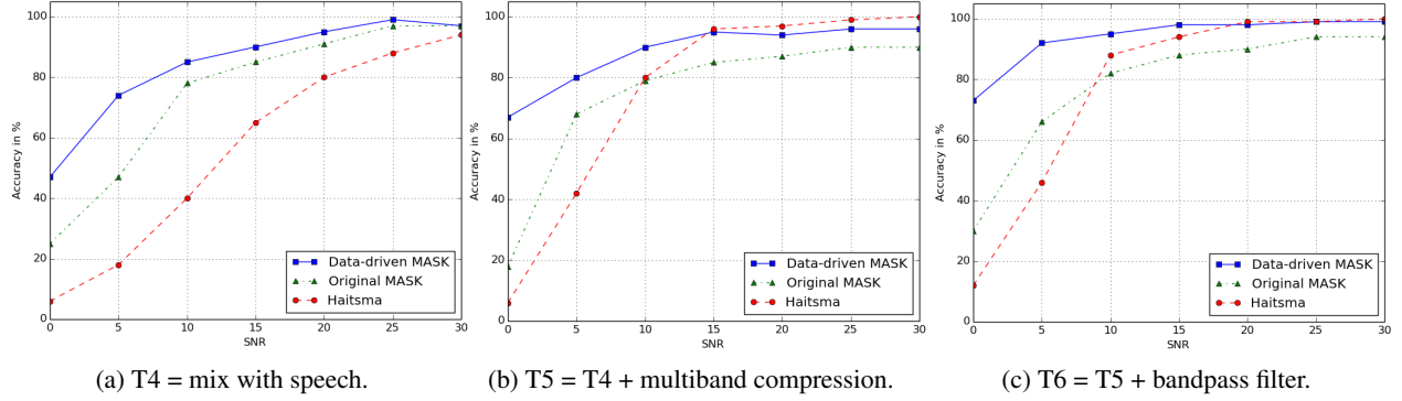
Fig. 3: Accuracies for 10 seconds queries for different SNR levels and acoustic transformations(T)
