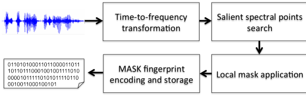
Fig. 1: MASK fingerprint extraction block diagram.
