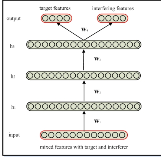
Fig. 3. DNN architecture.
