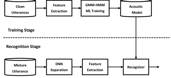
Fig. 2. Development flow for speech recognition system.
