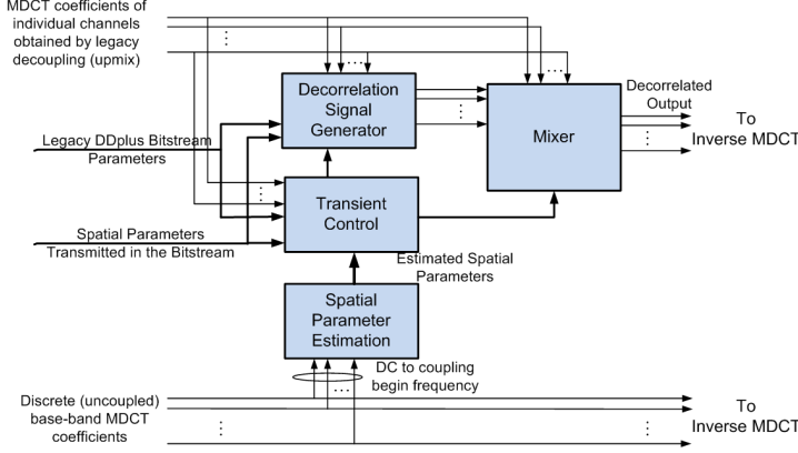
Fig. 1. Overview of the proposed MDCT-domain decorrelator for DDPlus
