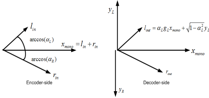
Fig. 2. Coupling two channels and upmixing with decorrelation
