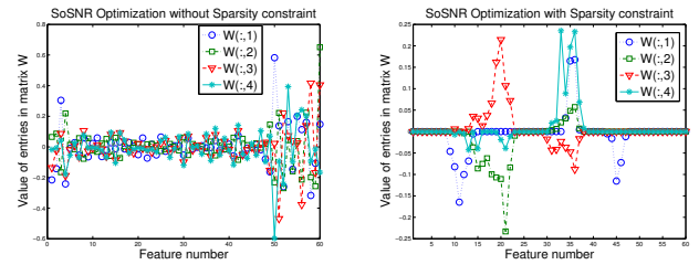
Fig. 5. Obtained \mathbf{W} with and without sparsity constraint.
