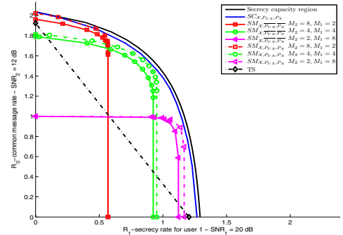
Fig. 4. Secrecy achievable rate regions with M = 8 and (SNR_1, SNR_2) = (16, 8) dB
