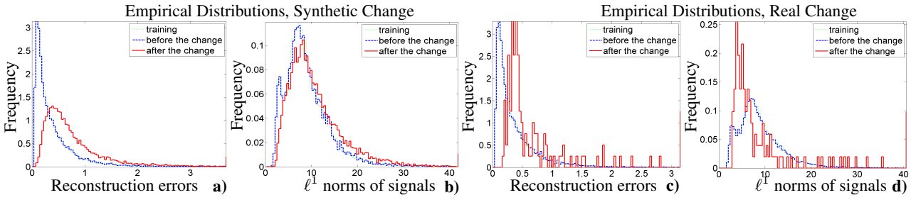
Fig. 2. Experiments on bursts dataset with synthetically induced change: (a), and (b), or simulating a real change by plugging 120 bursts recorded from a different deployment: (c) and (d). The distributions of the reconstruction errors in (a) (KS statistic value 0.42) and (c) (KS statistic value 0.45) clearly highlights the change, while it is more difficult to detect the change from the \ell^1 norms of the input signals (b) (KS statistic value 0.12) and (d) (KS statistic value 0.23).
