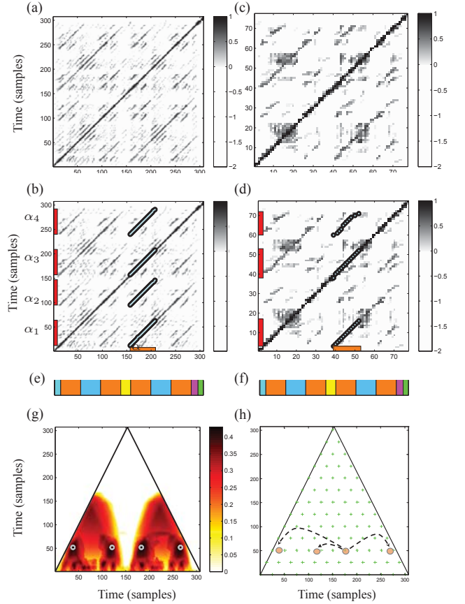
Fig. 3. Illustration of the fitness computation and possible risks of the reduction of the SSM resolution. (a) SSM with 2 Hz resolution. (b) Optimal path family for the segment \alpha = [158 : 209] using the SSM from (a). (c) SSM with 0.5 Hz resolution. (d) Optimal path family for the segment \alpha = [158 : 209] using the SSM from (c). (e)/(f) Ground-truth segmentation. (g) Fitness scape plot obtained from (a). The segment \alpha = [158 : 209] and all induced segments are indicated by circles. (h) Exploiting path relations for fitness estimation of the induced segments.
