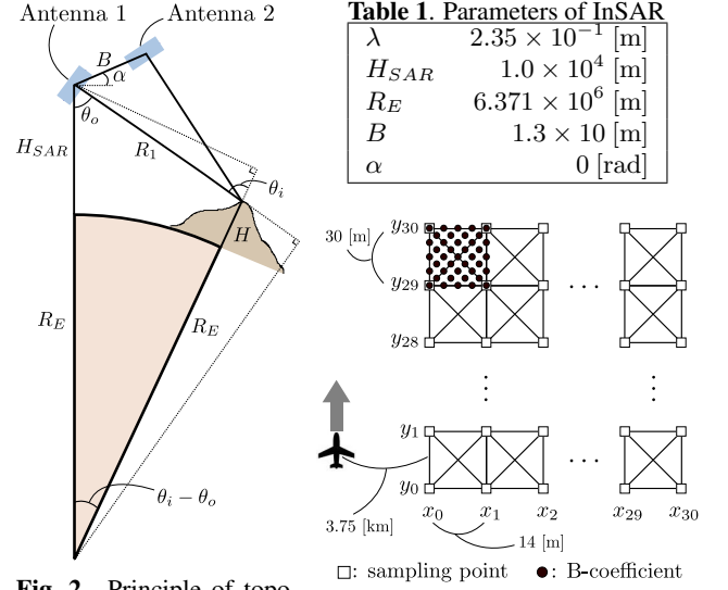
Fig. 2. Principle of topographic mapping by InSAR
