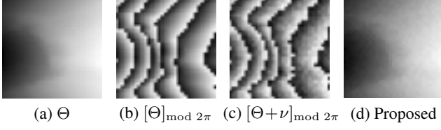
Fig. 4. Result of the proposed 2D phase unwrapping
