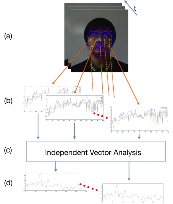
Fig. 2. Illustration of the proposed algorithm. (a) video sequence with detected landmarks and sub-regions. (b) 3 channel signals from 7 sub-regions (i.e. 7 groups). (c) IVA applied on the grouped signals. (d) 21 source signals recovered by IVA.
