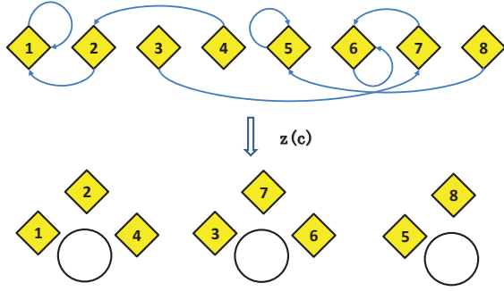
Fig. 1. An illustration of dd-CRP. The diamonds denote customers and the circles denote tables. The lines with arrow are the links between customers. In this example, the first customer c_1 links to itself. Customer c_2 links to c_1 , c_4 links to c_2 and no other costumers link to them. Hence c_1 , c_2 and c_4 sit at the same table.
