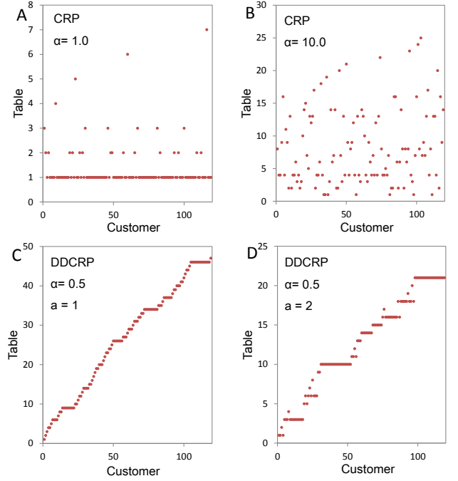
Fig. 2. Draws from CRP and dd-CRP. We can see that the draws of CRP (A and B) are dispersive, because CRP has no good property of segmentation. The draws of dd-CRP (C and D) form clear clusters according to the adjacent area in sequence data.
