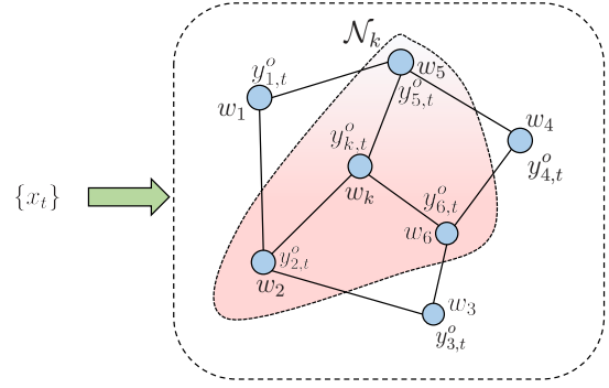
Fig. 1. Each agent is in charge of one dictionary element, w_k , and the corresponding coefficient, y_k , and the data sample x_t at each time t is available to all agents in the network. The results in this paper are generalized to the case where the data sample x_t is only available to a subset of the agents, and where each agent is responsible for a submatrix of W consisting of multiple columns and not only a single atom, w_k — see the extended work [17].
