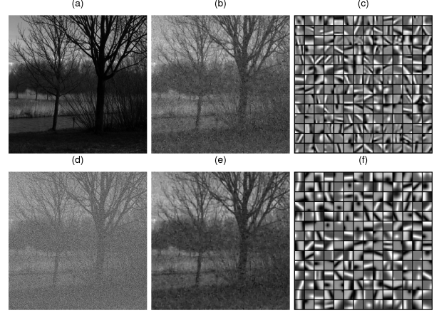
Fig. 3. Application of dictionary learning to image denoising. (a) Original image; (b) denoised image by using the centralized method from [2]; (c) dictionary obtained by the centralized method from [2]; (d) image corrupted by additive white Gaussian noise; (e) denoised image by our proposed distributed method at agent 1; (f) dictionary obtained by our proposed distributed method.
