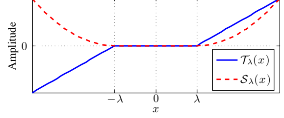
Fig. 2. Illustration of the functions \mathcal{T}_{\lambda}(x) and \mathcal{S}_{\lambda}(x) .
