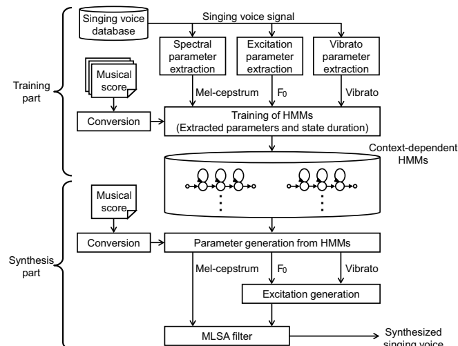
Fig. 1. Overview of HMM-based singing voice synthesis system.
