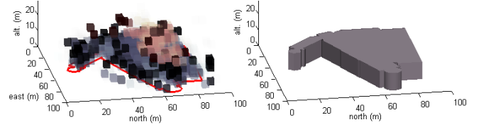
Fig. 6. Left: 3D occupancy map around Kohn Hall, with cell transparency set to emptiness probability (i.e., areas assigned low occupancy probabilities are transparent), and red tinted cells being those above 12 m. Right: approximate ground truth based on OSM data.
