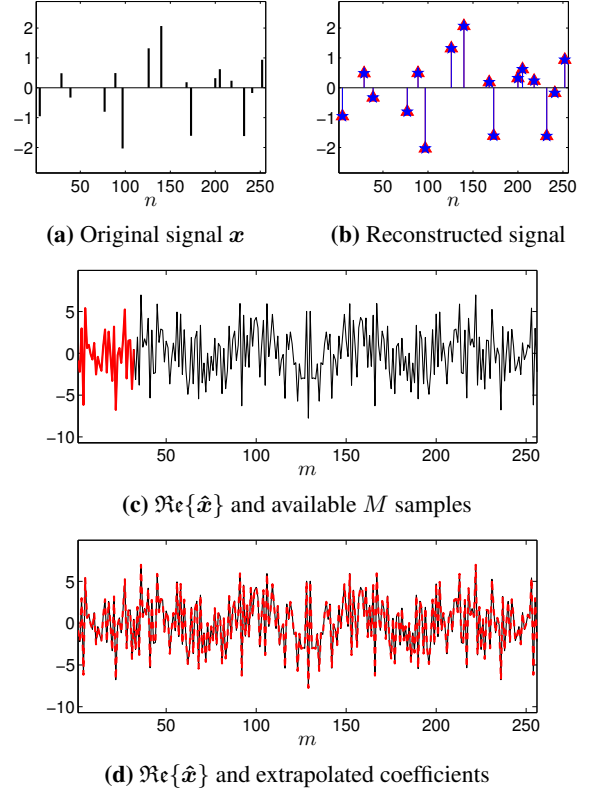
Fig. 1: N = 256 , M = 32 and K = 16 . (a) Signal with K = 16 Diracs. (b) Perfect reconstruction of the signal, in red the original signal and in blue the reconstruction. (c) Real part of the Fourier coefficients in black and available samples in red. (d) Real part of the Fourier coefficients in black and extrapolated coefficients using the method in Proposition 1, in red.
