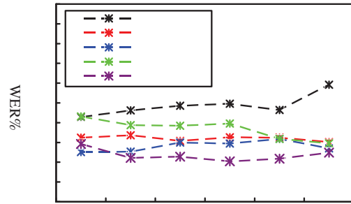
Figure 3. Performance of SGMM and SMM on 3 hour training data as the number of substates increases.
