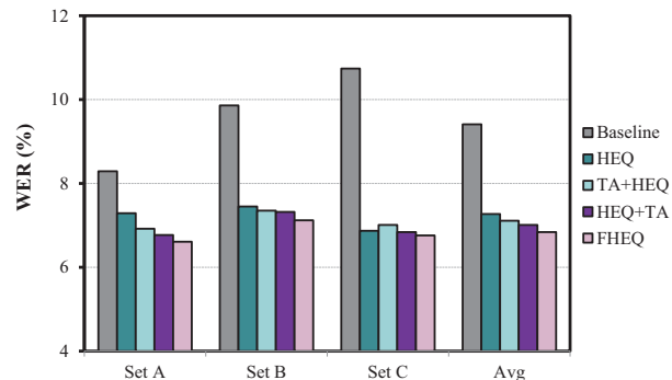
Fig. 3. WER (%) of the MFCC baseline, HEQ, TA+HEQ, HEQ+TA, and FHEQ on the Aurora-2 task.
