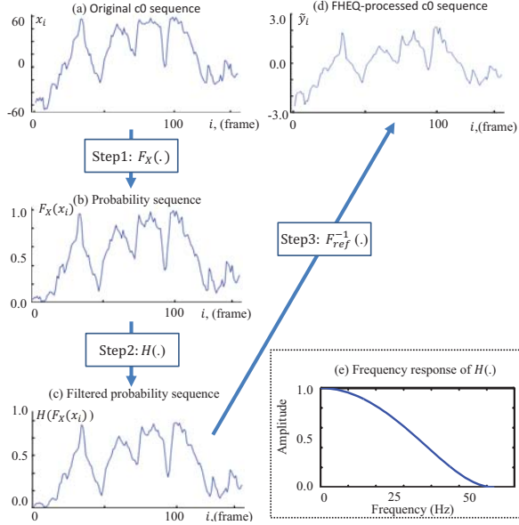
Fig. 2. Procedure of the FHEQ algorithm
