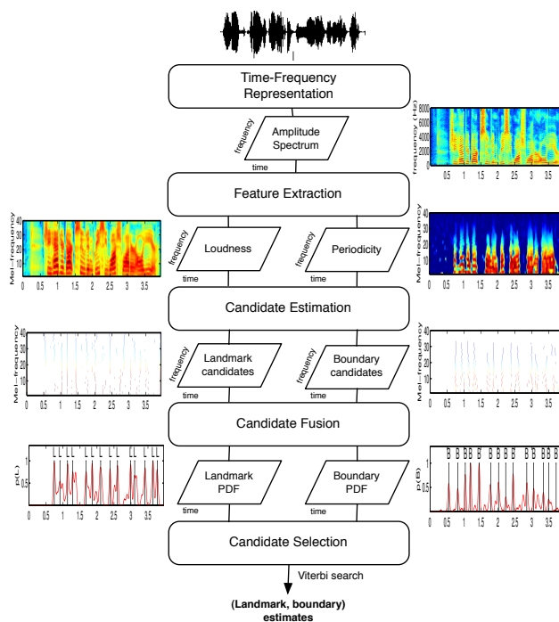
Fig. 1. Overview of the SYLL-O-MATIC system.
