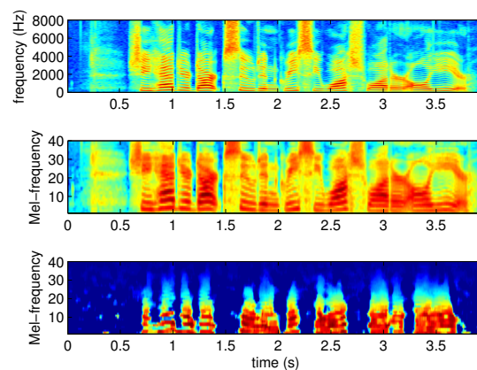
Fig. 2. Spectrogram, specific loudness, and voiced/unvoiced representations for the SA1 utterance : "She had your dark suit in greasy wash water all year." spoken by FAKS0 speaker.
