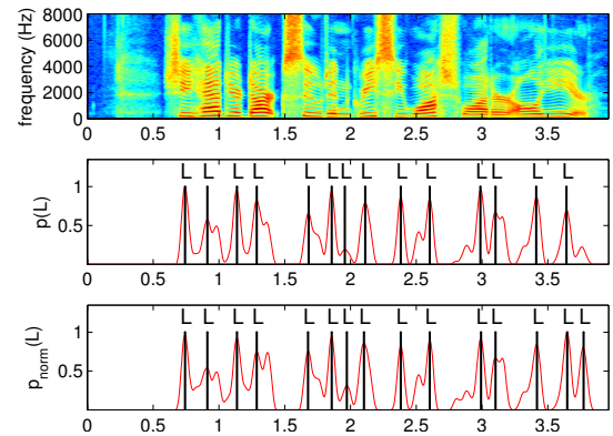
Fig. 5. Landmarks PDFs and the determined sequence of landmarks (L) with (bottom) and without (middle) the selection of useful frequency regions for the SA1 utterance : “She had your dark suit in greasy wash water all year.” spoken by FAKS0 speaker.
