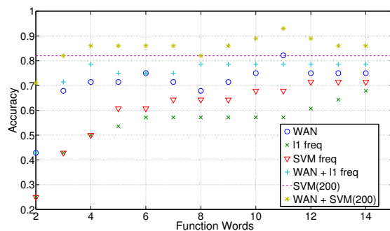
Fig. 2. Accuracy as a function of function words for a problem with 8 authors and 4 known texts per author [20]. The accuracy of the WAN method developed is higher than that of a frequency based SVM and a frequency based l1 norm for this range of function words. The accuracy of the combined methods is higher than that of their constituent methods indicating that relational and frequency based information encode different stylistic features.
