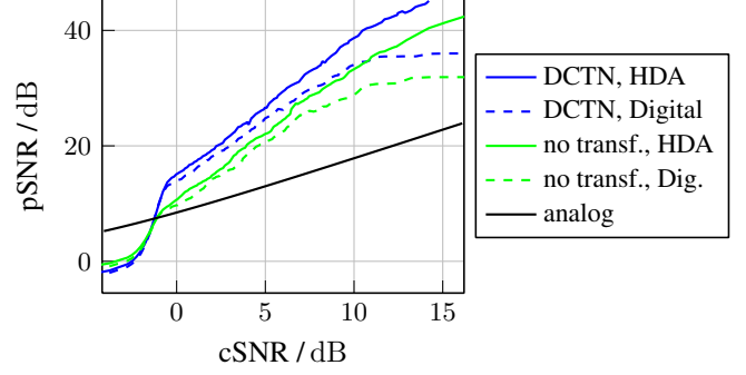
Fig. 4. Envelopes for HDA and digital transmission for a Gaussian source with \rho = 0.8 . Simulations with Turbo coding and with and without DCTN transform. 2 \leq F_D \leq 6 , 1.66 \leq F_H \leq 5 , M = 128 , L = 128 , N = 768 . Purely analog transmission system for comparison.
