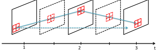
Fig. 1: Trajectory of interpolated pixels across frames when motion compensation is performed (continuous arrow) and when it is not (dashed arrow).
