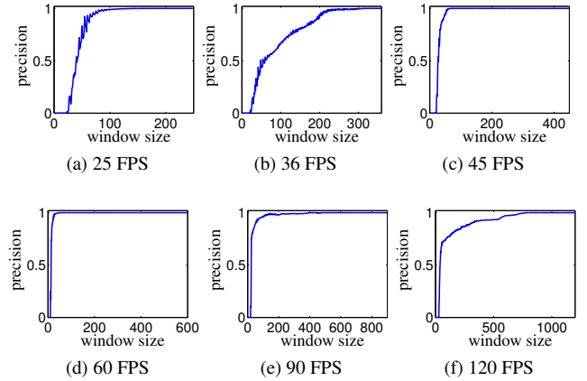
Fig. 3: Precision for different temporal window size (number of frames).
