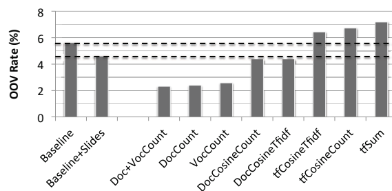
Fig. 1. Average OOV rate for different features
