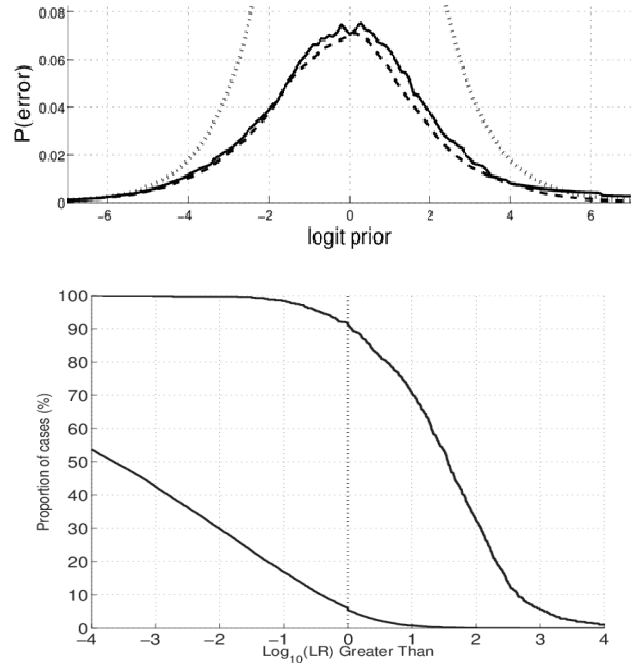
Figure 2. APE and Tippet plot of elicited LRs from a single phone system (phone IY) in the SRE04 English 1s1side task with session variability compensated MFCC trajectories.
