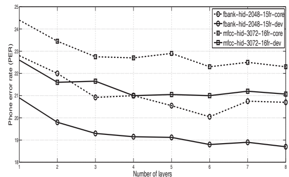
Fig. 2. PER as a function of the number of layers.
