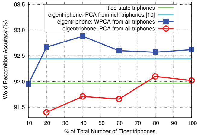
Fig. 1. Effect of weighted PCA and eigentriphone pruning using bigram LM.
