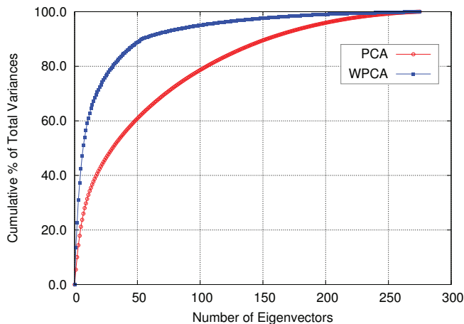
Fig. 3. Eigenspectra obtained from weighted PCA and conventional PCA for the base phoneme [aa].
