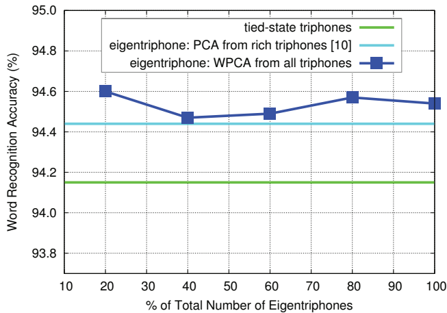
Fig. 2. Effect of weighted PCA and eigentriphone pruning using trigram LM.
