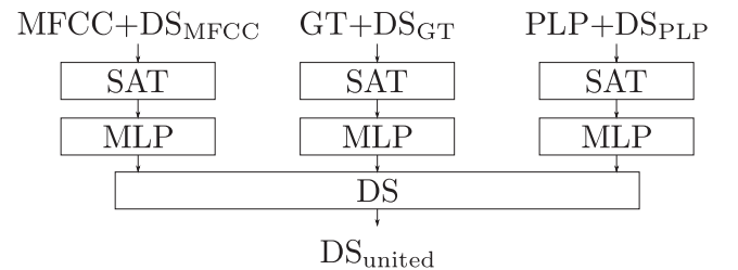
Fig. 1. Combination of different CRBE based features in posterior feature space after speaker normalization
