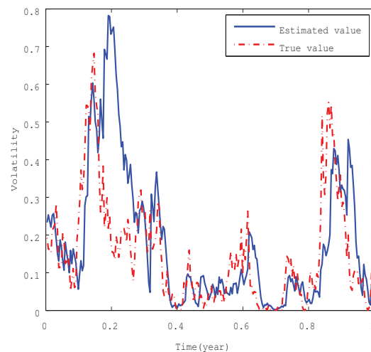
Fig. 2. True and estimated v_t
