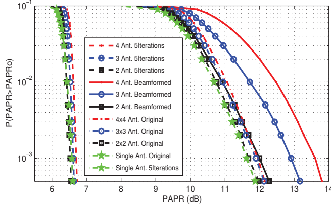
Fig. 2: CCDF curves of PAPR for 64QAM OFDM block with N = 1024 and M = 60 . The curves are plotted for different number of antennas and T = 2 . Corresponding PAPR reduced CCDFs are derived with 5 iterations.
