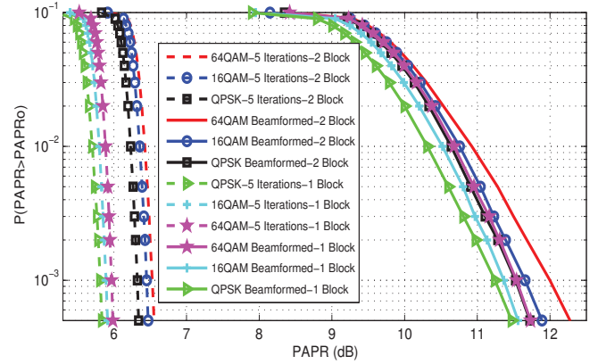
Fig. 3: CCDF curves of PAPR for 2 \times 2 MIMO OFDM block with N = 1024 and M = 60 . The curves are plotted for different constellations and T = 1, 2 .
