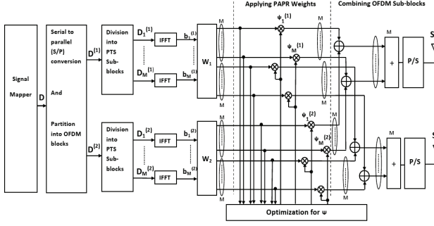
Fig. 1: Block diagram of MIMO-PTS technique for two antennas. The input data block \mathbf{D} is partitioned into two M disjoint sub-blocks such that \sum_{m=1}^M \mathbf{D}_m^{(q)} = \mathbf{D}^{(q)} . Known beamforming weights \mathbf{w}_1 and \mathbf{w}_2 are multiplied with first and second OFDM sub-blocks, respectively to produce the contributing signal for the first (upper) and second (lower) antennas. Then, phase weights \psi_m^{(q)} = e^{j\phi_{q,m}} are multiplied with all sub blocks. The relevant sub blocks are summed to form the final OFDM sequences on both antennas.
