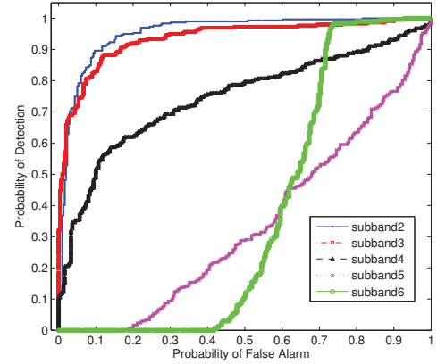
Fig. 5. ROC curve showing the performance of the second step of our detection technique. This step detects the images acquired by compressive sensing and separate them from those compressed using a DWT-based technique.
