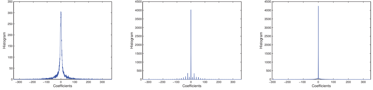
Fig. 1. Histogram of DWT coefficients taken from uncompressed Lena (left), the same image after JPEG2000 compression (center), and the reconstructed compressively sensed Lena (right).
