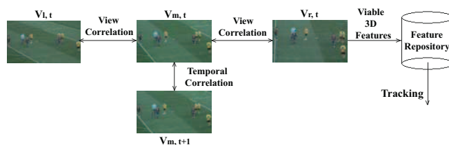
Fig. 1. SIFT-based tracking scheme.
