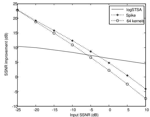
Fig. 3. SSNR evaluation of spike coding based enhancement
