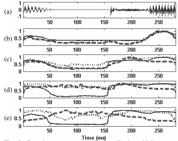
Fig. 2. Gaussian parameter tracks (amplitude - thick, mean - dashed, and variance - dotted): (a) waveform of /apa/ , (b) Gaussian 1, (c) Gaussian 2, (d) Gaussian 3, and (e) Gaussian 4.
