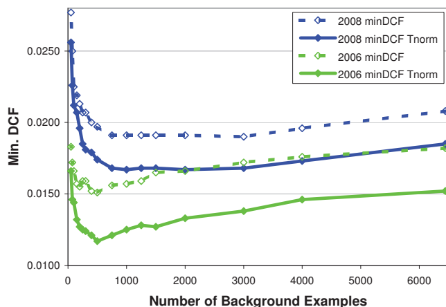
Fig. 1. Un-normalised and T-normed min. DCF on 1-sided, English NIST 2006 and 2008 SRE as the background dataset is refined.
