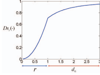
Fig. 2. Spatial distance D_{Si}(\mathbf{x}_k^i, \hat{\mathbf{x}}_k^{i,q}) .
