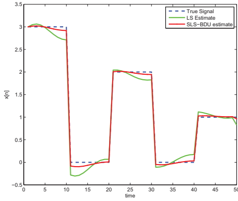
Fig. 2. Actual and restored signals are shown in dashed and solid lines respectively.
