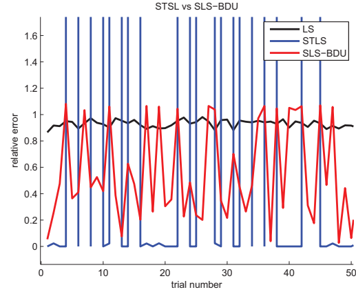
Fig. 3. Relative Estimation Error of LS, STLS and SLS-BDU in 50 independent trials. Frequently \|x_{STLS}\| attains huge values because of ill conditioning.
