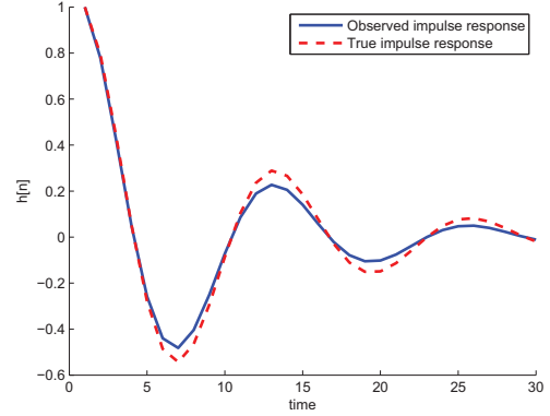
Fig. 1. Nominal and actual impulse responses are shown in solid and dashed lines respectively.
