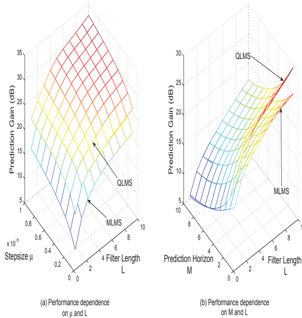
Fig. 1. The performance of Quaternion LMS and multi-channel LMS on the prediction of 3D Lorenz signal.
