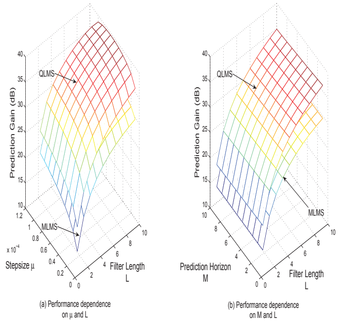
Fig. 2. The performance of Quaternion LMS and multi-channel LMS on the prediction of 3D wind field coupled with temperature.
