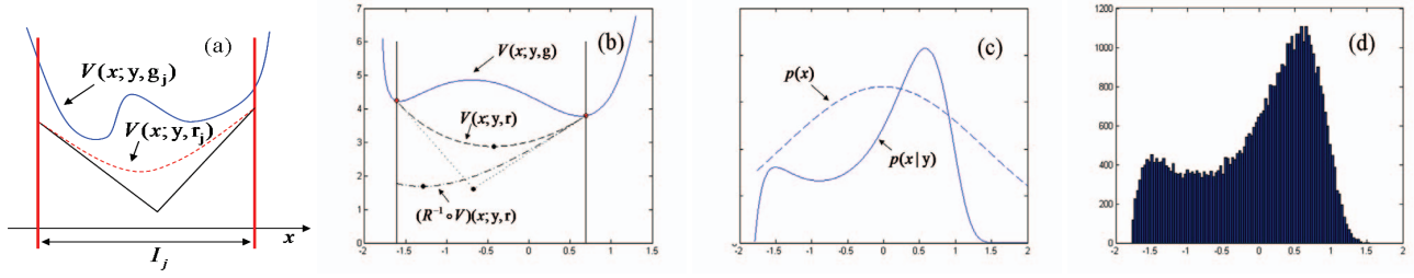
Fig. 2. (a) The intersection of the tangents to V(x; \mathbf{y}, \mathbf{r}_j) at \min(\tilde{X}_j) and \max(\tilde{X}_j) is a lower bound for V(x; \mathbf{y}, \mathbf{g}_j) . (b) The system potential V(x, \mathbf{y}, \mathbf{g}) (solid), the modified system potential V(x, \mathbf{y}, \mathbf{r}) (dashed), function (R^{-1} \circ V)(x, \mathbf{y}, \mathbf{r}) (dot-dashed) and two tangent lines (dotted). (c) The target density p(x|\mathbf{y}) (solid), and the prior p(x) (dashed). (d) The histogram of N = 10000 samples using RS.
