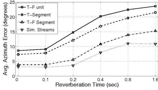
Fig. 2. Average azimuth estimation error at four T-F grouping levels: T-F unit, T-Segment, Segment and Simultaneous Stream.
