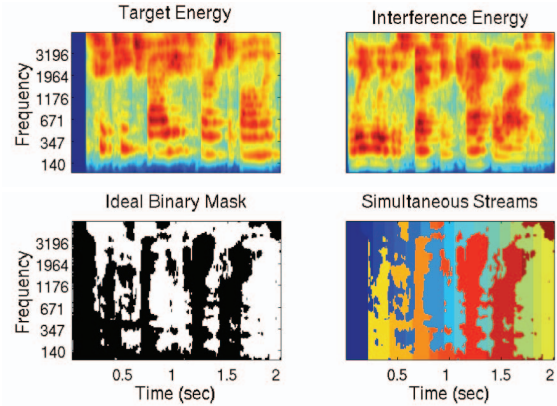
Fig. 1. Illustration of the formation of T-F objects. (top left) Cochleagram of target signal. (top right) Cochleagram of interference signal. (bottom left) Ideal binary mask for target signal where 1 is white and 0 is black. (bottom right) Simultaneous streams created with IBM and manual labeling of syllable boundaries.
