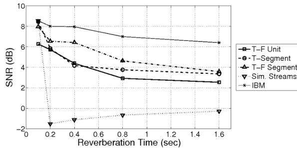
Fig. 3. SNR output for four T-F grouping levels and IBM.
