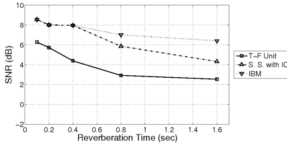
Fig. 4. SNR output for T-F unit level, simultaneous stream level including interaural coherence and IBM.
