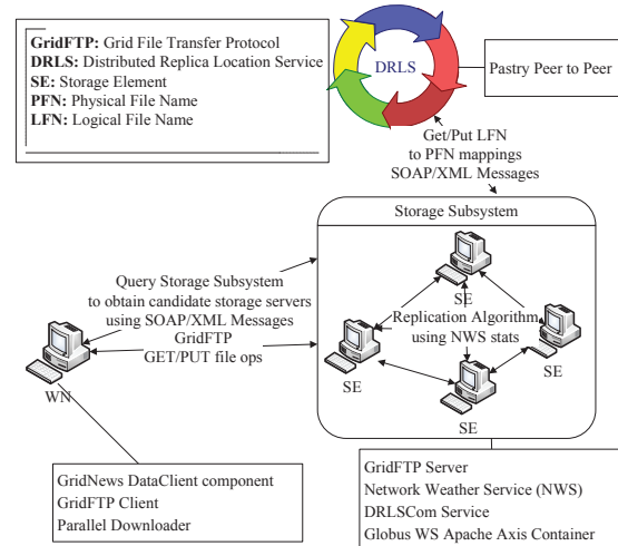
Fig. 3. Storage architecture
