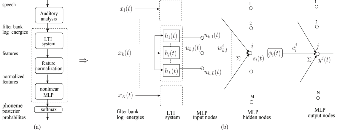
Fig. 1. (a) Estimation of posterior probabilities of phonemes using an MLP. (b) Part of the system that is analyzed using Volterra series.
