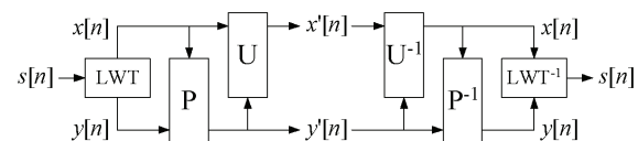
Fig. 1. Generalized Lifting Scheme
