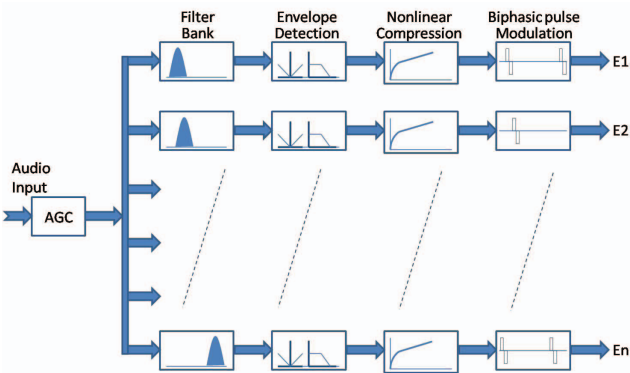
Figure 3: CIS Algorithm
