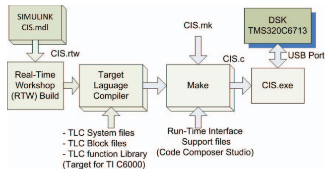
Figure 5: DSP Code generation routine from SIMULINK
