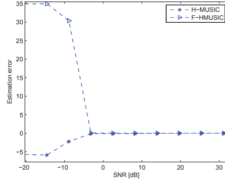
Fig. 3. The order estimation errors calculated using F-HMUSIC and HMUSIC with the white noise.
