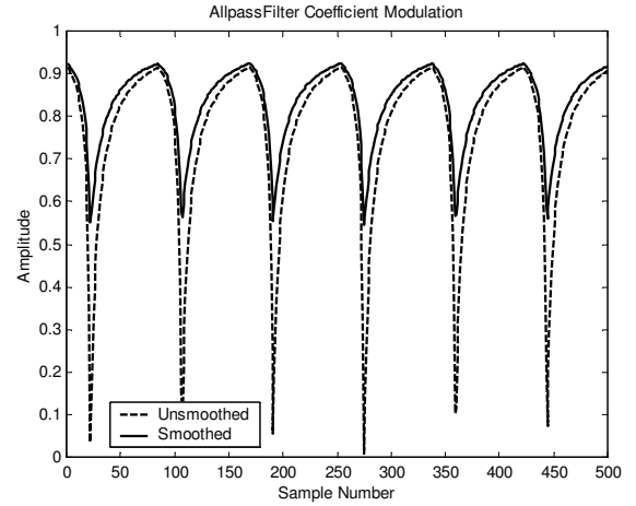
Fig.4. Coefficient modulation function from phase distortion sawtooth
