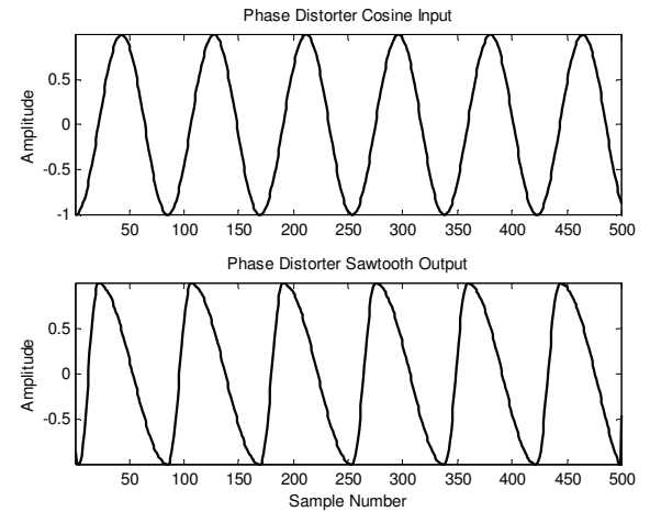
Fig. 2. Input cosine and output sawtooth of phase distorter
