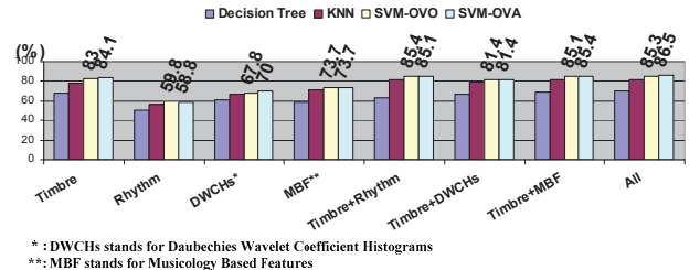
Fig. 2. Accuracy of six-style classification
