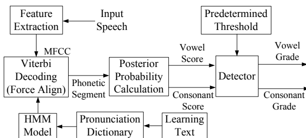
Fig. 1. Architecture of our pronunciation evaluation system
