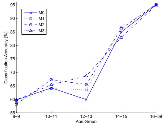
Fig. 2. Gender classification accuracy for each age group using the measures sets M1, M2 and M3. M0 represents the baseline performance results. The corresponding values are listed in Table 4.
