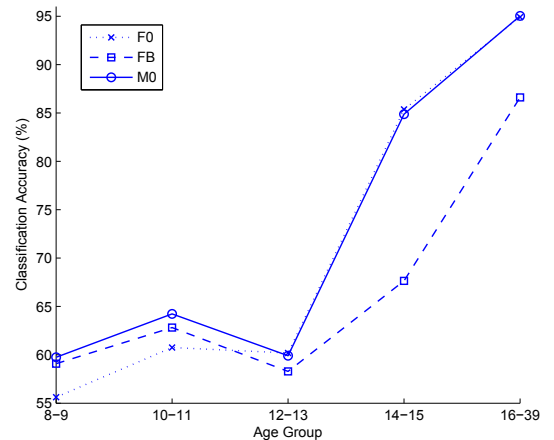
Fig. 1. Gender classification accuracy for each age group using just F_0 , just FB, and F_0 plus FB (M0).
