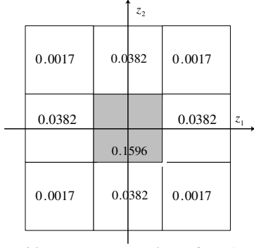
Fig. 1. LM with 2 parameters: values of E1 (central square) and E2 (all other squares). The edge length of each square is 2\sqrt{3} .
