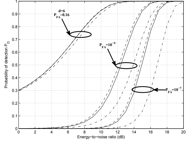
Fig. 2. Performances for sinusoidal detection: GLRT (solid line), best results of ODD (dashed line), worst results of ODD (dashdot line).
