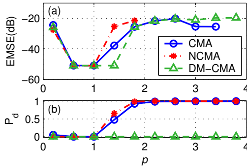
Fig. 5. (a) EMSE and (b) P_d as a function of the initialization \mathbf{pw}_o , where \mathbf{w}_o^T = [-0.005 \ 0.016 \ -0.047 \ 0.140 \ -0.417 \ 1.250 \ -0.417 \ 0.138 \ -0.046 \ 0.016 \ -0.005] ; h_0 = 0.3 in the absence of noise, 2-PAM, N = 10^4 , L = 10^3 , \mu = 0.037 , \tilde{\mu} = 1 , M = 11 , \delta = 10^{-5} .
