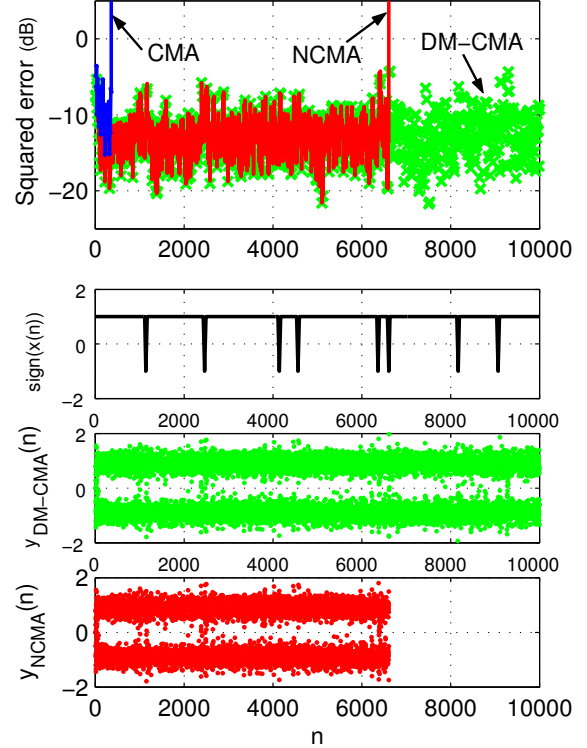
Fig. 2. Squared error in dB ( e^2(n) ) for CMA and DM-CMA, sign of x(n) for DM-CMA and output of the equalizer for DM-CMA and NCMA; 2-PAM, h_0 = 0.3 , SNR = 20 dB, \mu = 0.044 , \tilde{\mu} = 1 , \delta = 10^{-5} .
