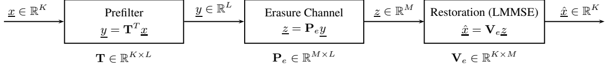
Fig. 1. Erasure Channel
