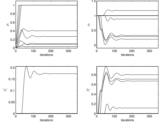
Fig. 1. Convergence of powers and Lagrange multipliers.
